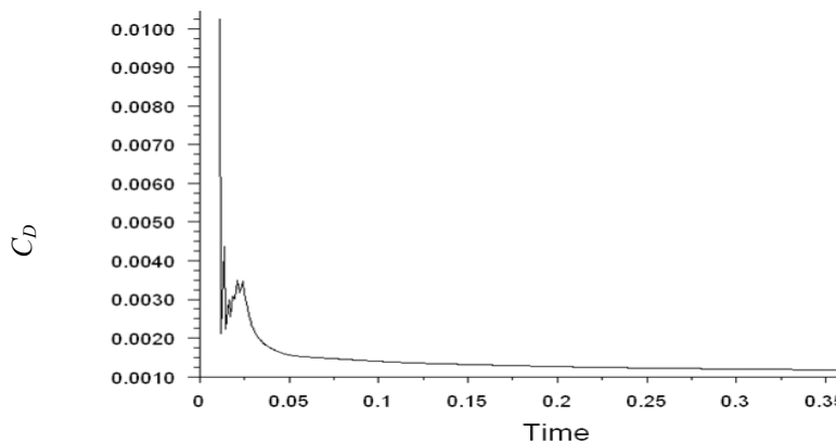
Figure 3: Drag convergence history
