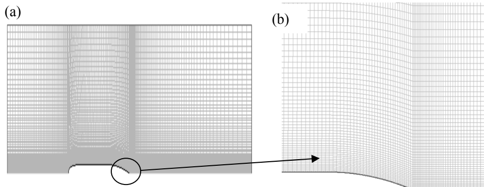
Figure 2: (a) Grid of flow domain around DREA bare submarine hull (b) Enlarged view of grid near stern side
