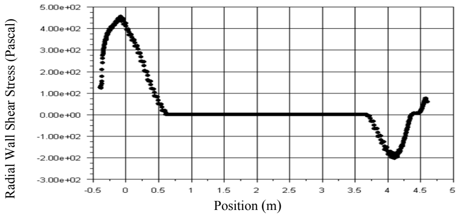
Figure 14: Variation of radial wall shear stress on AUV ( L/D=6 )
