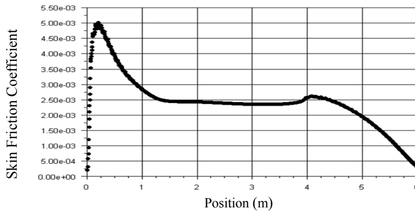
Figure 9: Variation of skin friction coefficient on the surface of DREA
