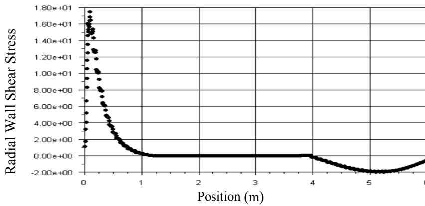
Figure 8: Variation of radial wall shear stress for DREA
