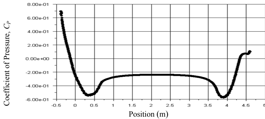
Figure 12: Variation of pressure coefficient around AUV ( L/D = 6 )
