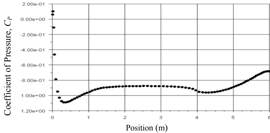
Figure 6: Variation of pressure coefficient, C_p around bare submarine hull DREA
