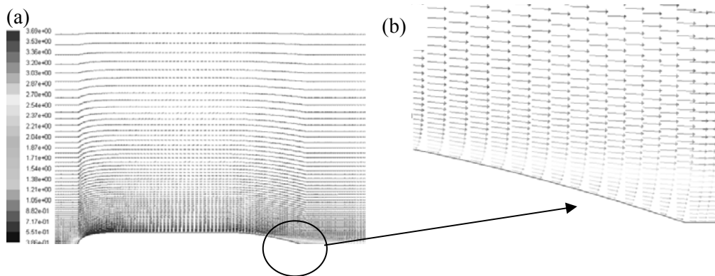
Figure 5: (a) Plot of velocity vectors around DREA (b) enlarged view of velocity vectors near stern
