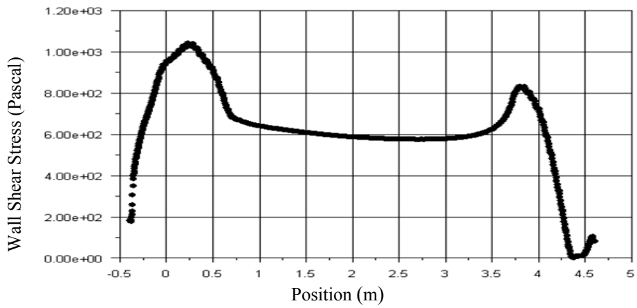
Figure 13: Variation of wall shear stress on AUV ( L/D=6 )
