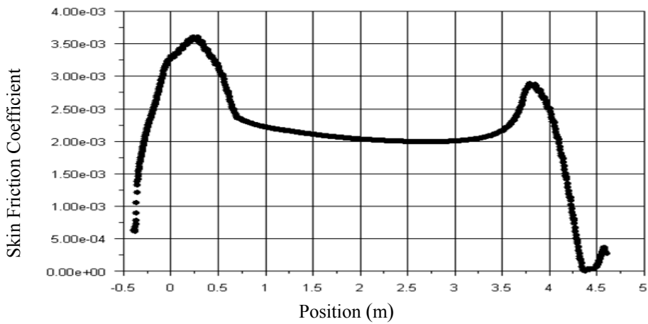
Figure 15: Variation of skin friction coefficient on AUV ( L/D=6 )
