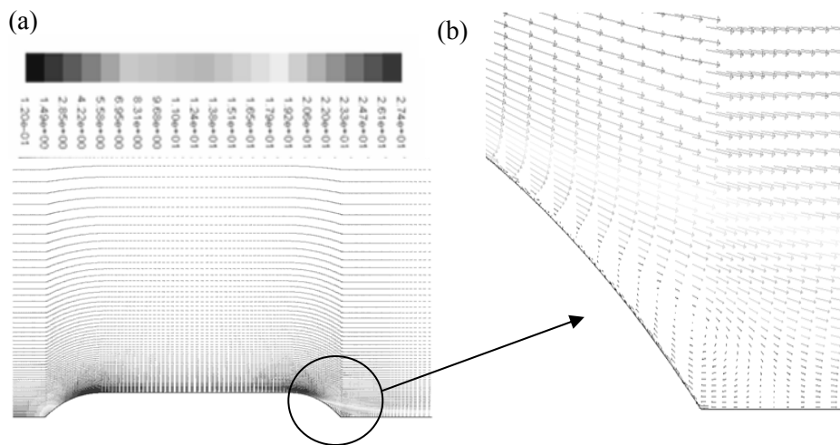
Figure 11: (a) Plot of velocity vector (b) Enlarged view of velocity vector near body
