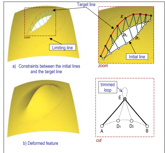
Figure 14: Insertion of G^1 discontinuity along the target line.
